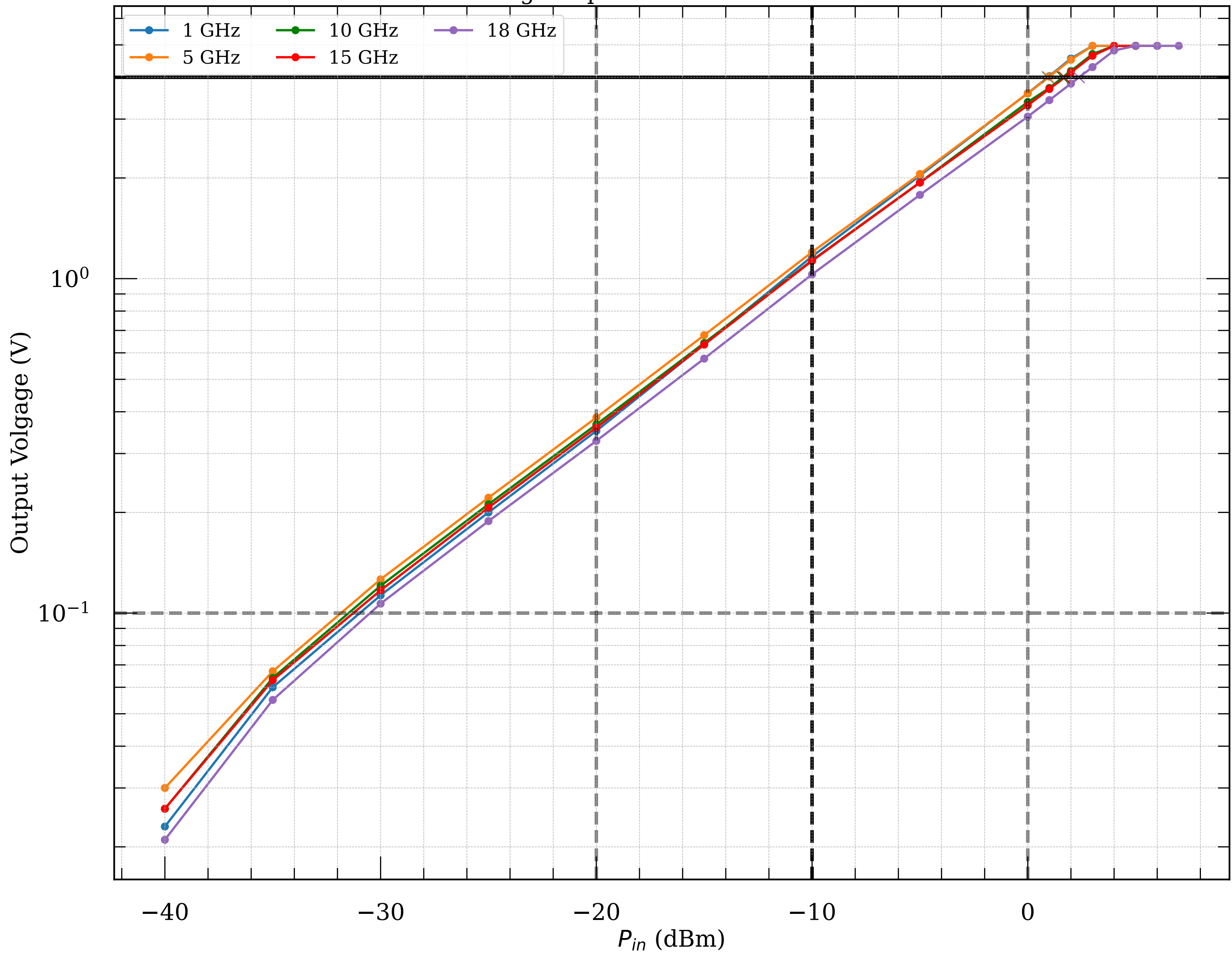
Measured voltage-to-power curve of detector module097
